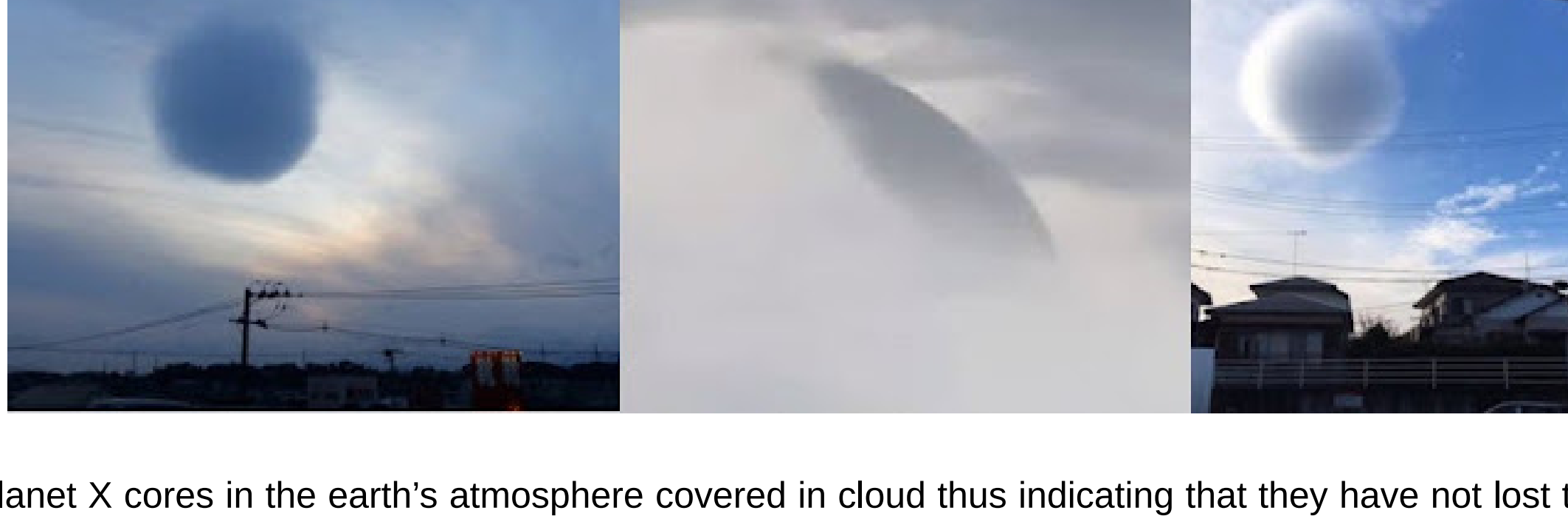
Figure 4. Planet X cores in the earth's atmosphere covered in cloud thus indicating that they have not lost their ability to generate a gravitational field, which manifests as a stationary density (sound) wave around their surfaces. They are suspended in the air suggesting that they are repelled away from the earth's surface, something which does not happen once they die, as then they fall and impact the ground [Article 1814: Planet X in the sky: gravity creates cloud].
